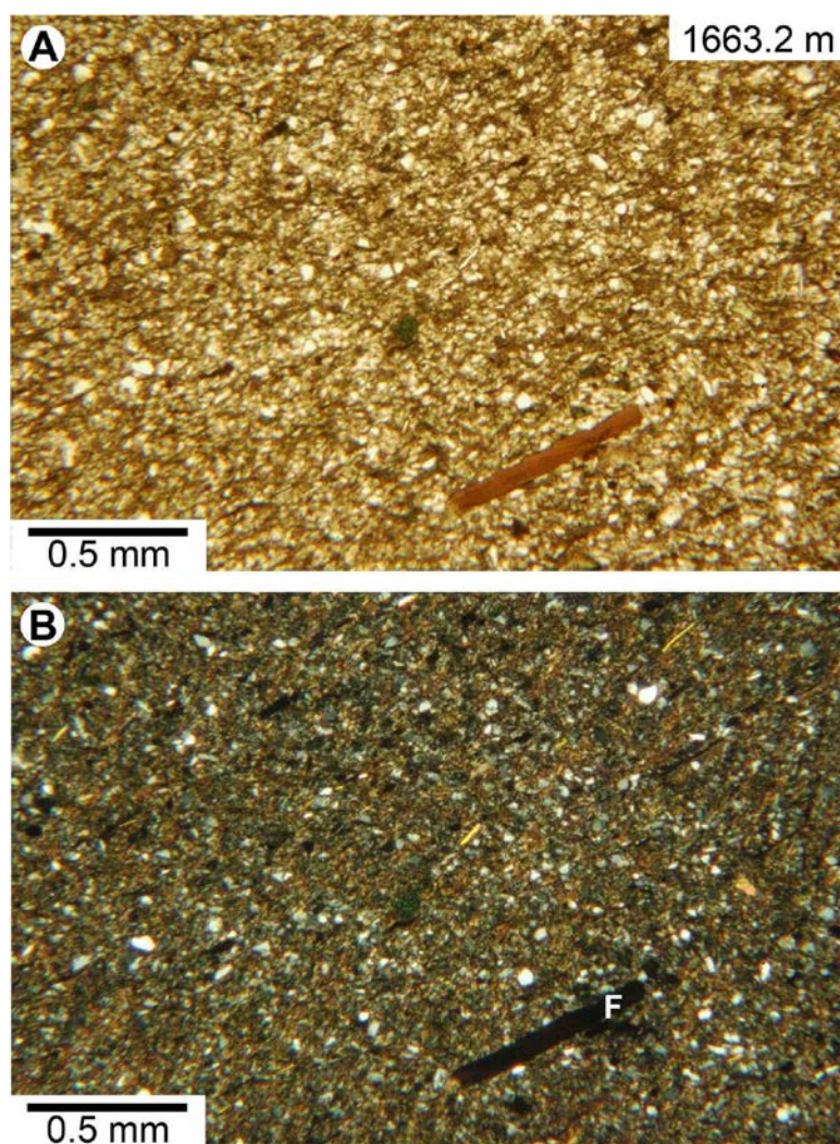
Figure A1. Photomicrographs of Eau Claire Shale cap rock (from a depth of 1,663.2 m). A, viewed in plane-polarized light; B, the same view under crossed polarizers. The fossil, labeled F in photomicrograph B, is oriented parallel to bedding in the shale. The rock is fine grained, and the pore spaces are filled with authigenic clays that substantially reduce porosity and permeability.
