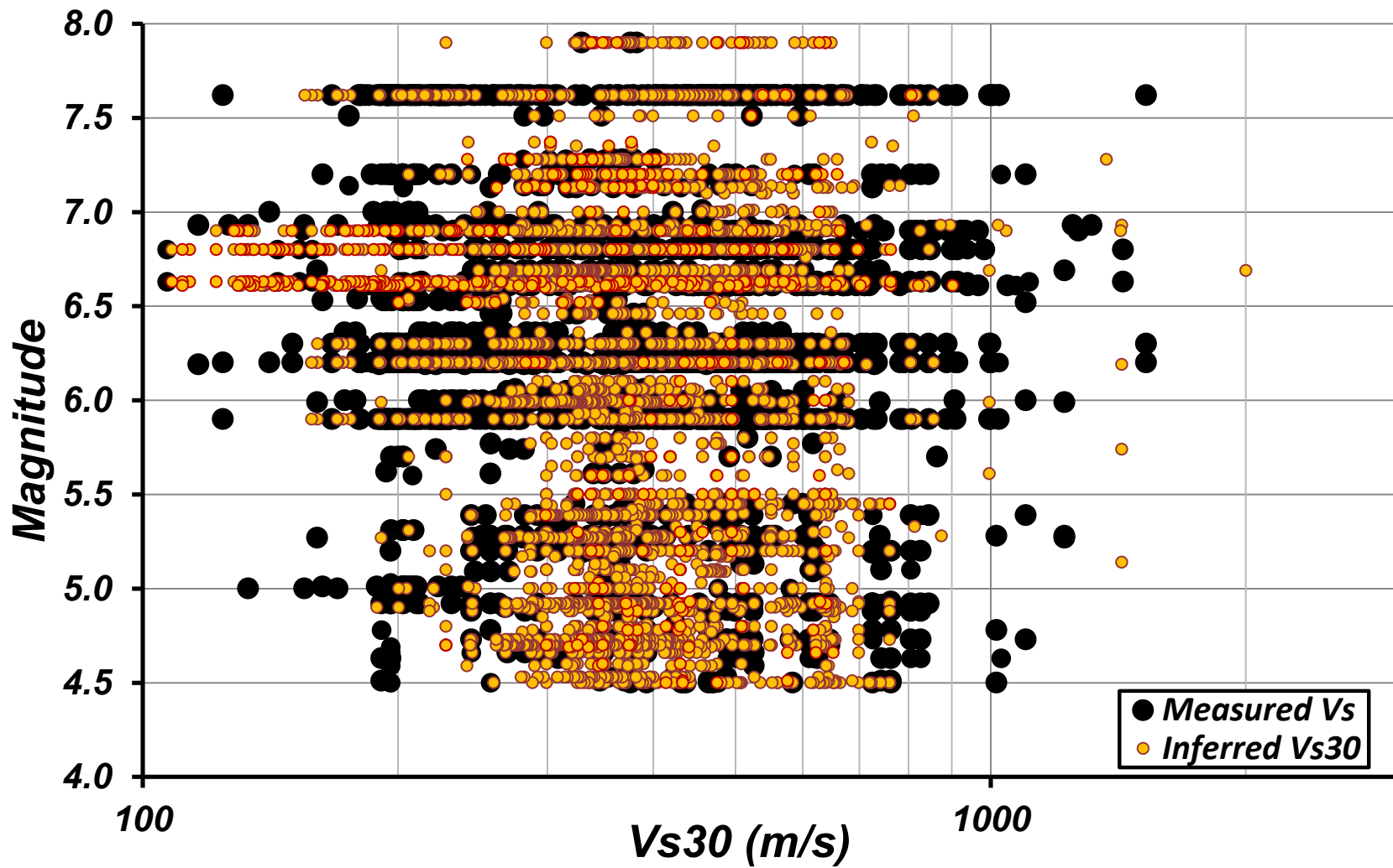
Magnitude versus V_{s30} -- free-field recordings
