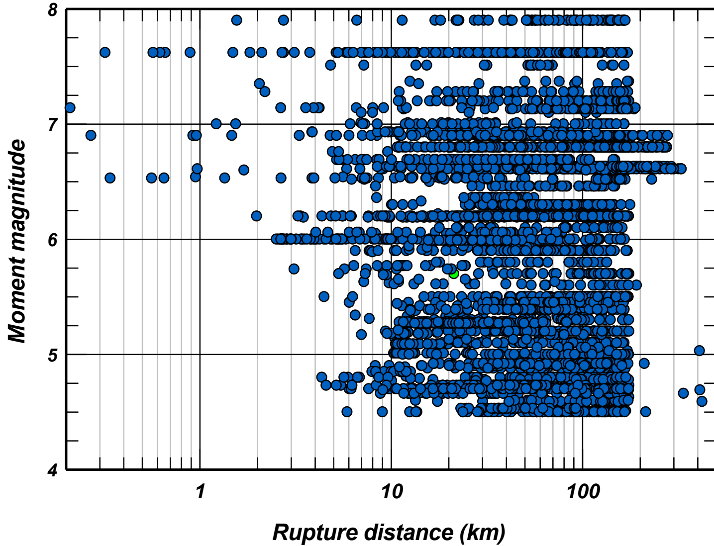
Magnitude versus Distance -- free-field recordings
