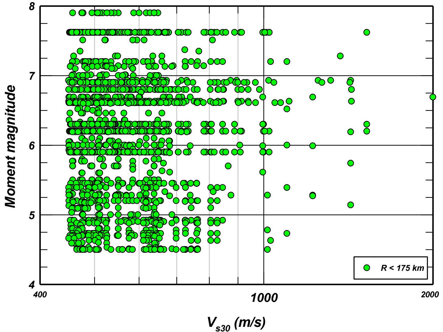
Magnitude versus V_{s30} -- free-field recordings R \leq 175 km; V_{s30} \geq 450 m/s
