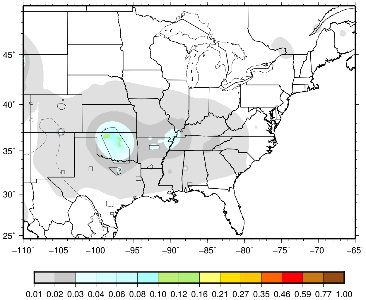
Spectral response acceleration for 1hz, expressed as a fraction of standard gravity (g) for 1% probability of exceedance in one year and Vs30 site condition of 760 meters per second
