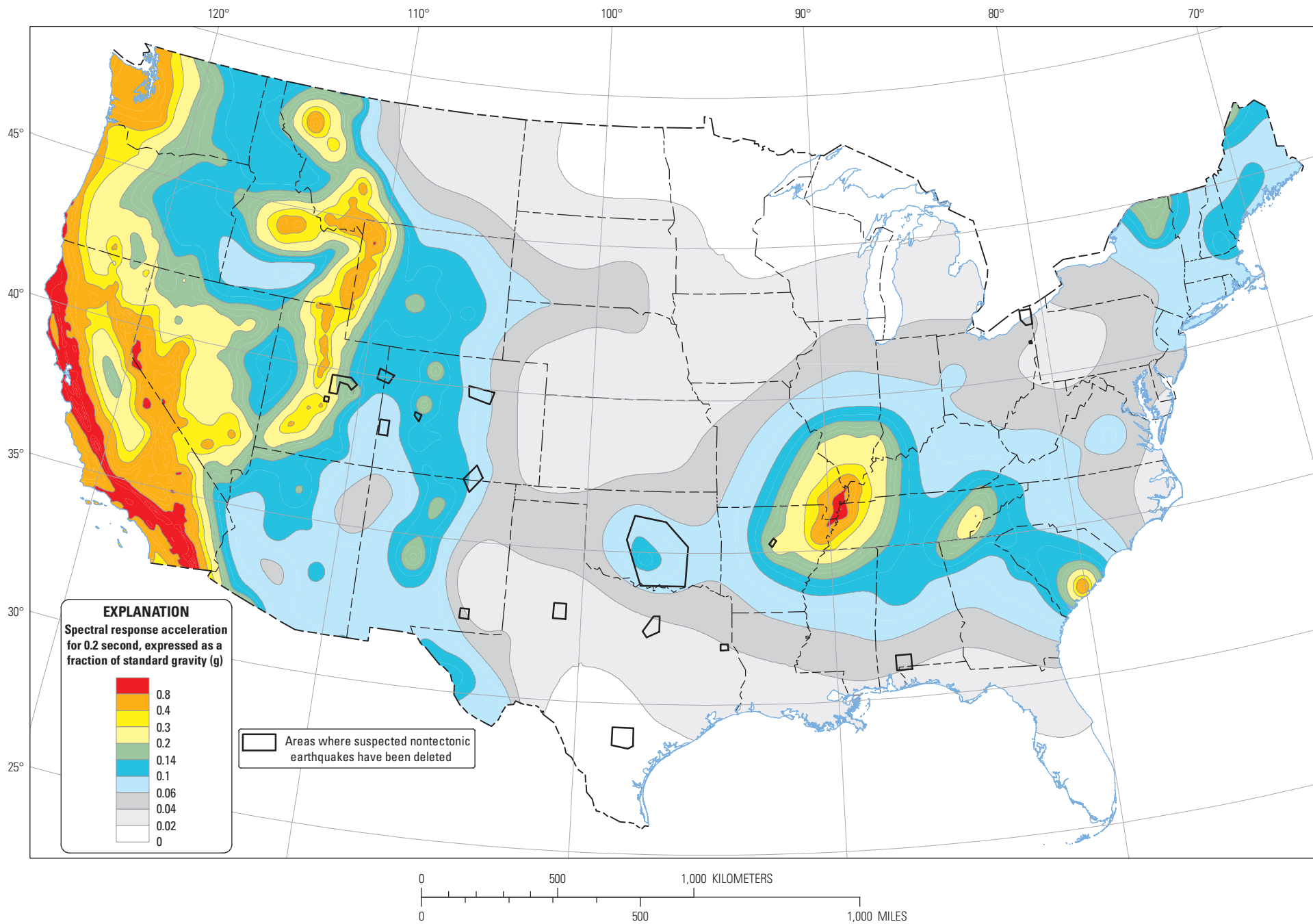
Ten-percent probability of exceedance in 50 years map of 0.2 second spectral response acceleration
