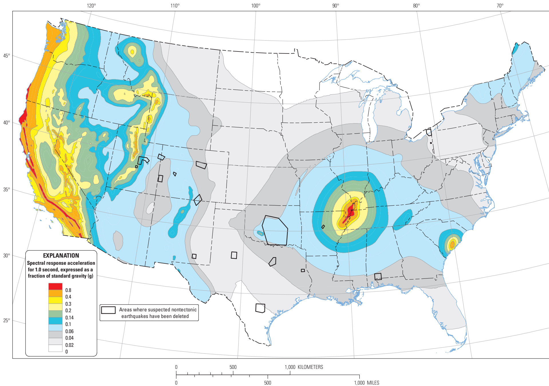
Two-percent probability of exceedance in 50 years map of 1.0 second spectral response acceleration
