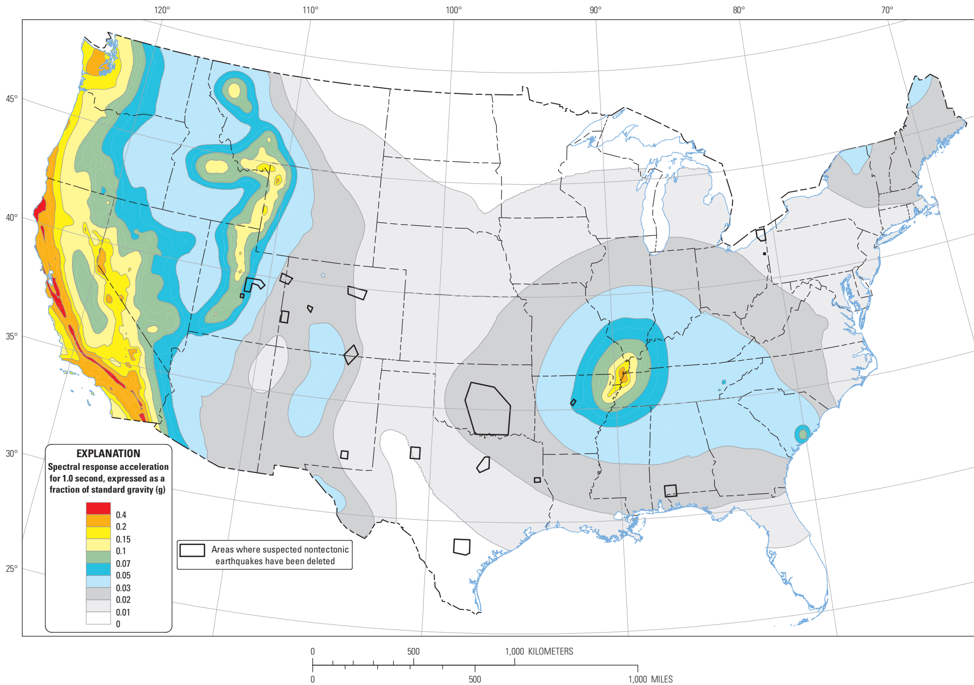
Ten-percent probability of exceedance in 50 years map of 1.0 second spectral response acceleration
