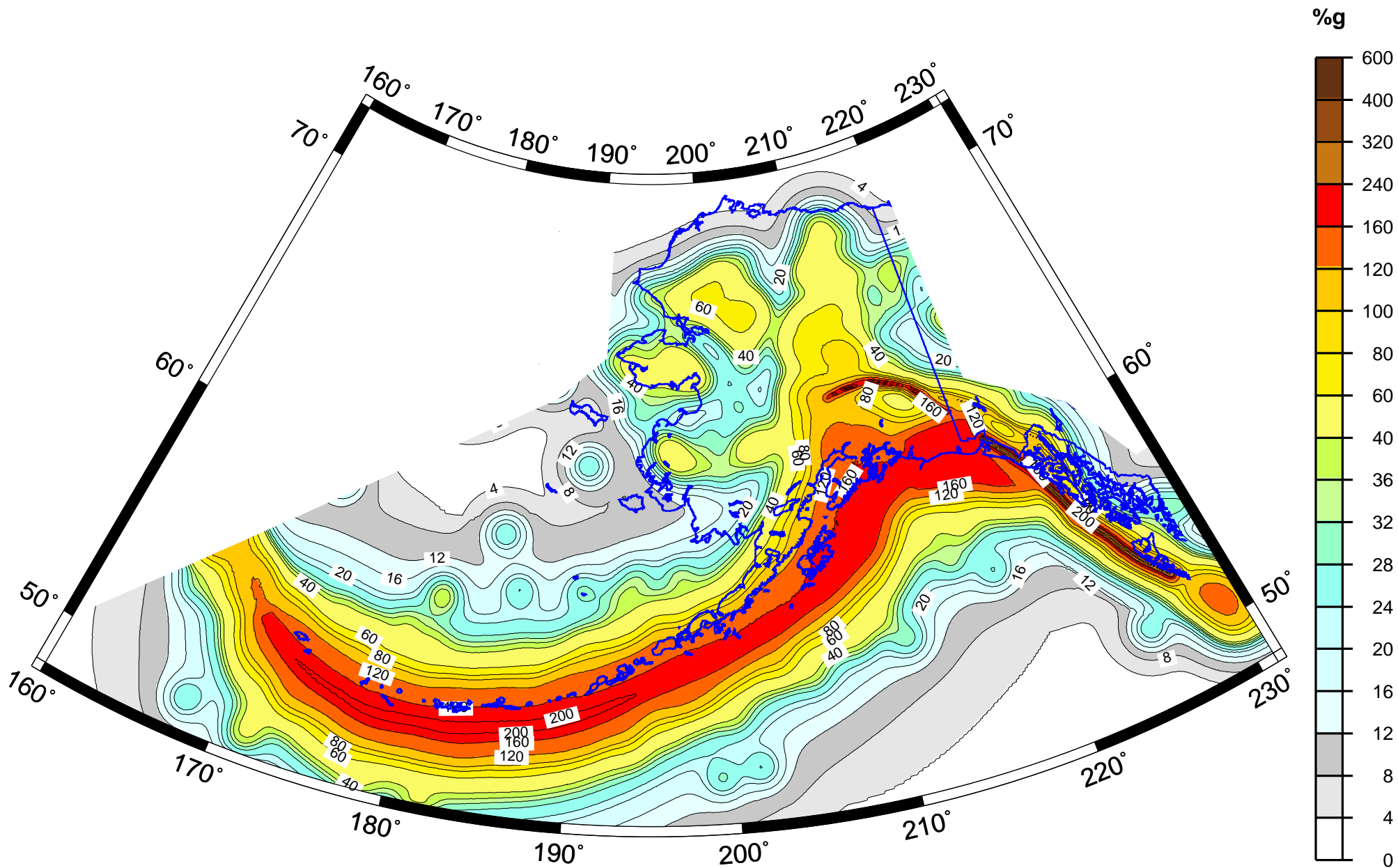
3 Hz Spectral Acceleration (%g) with 2% Probability of Exceedance in 50 Years
