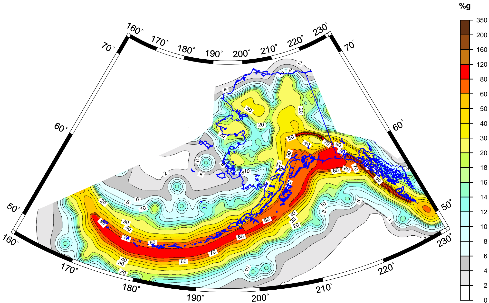
Peak Ground Acceleration (%g) with 2% Probability of Exceedance in 50 Years
