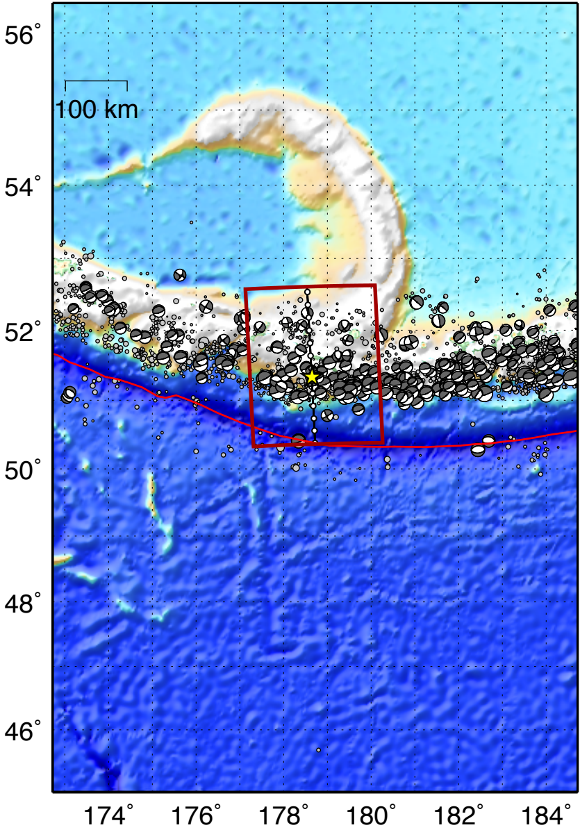
Rat: 05/20/2008 Mw 6.0 Rat Islands Earthquake Cross-section Width = +/- 100km (Most Likely Depth if on planar slab interface = 37.4 km)
