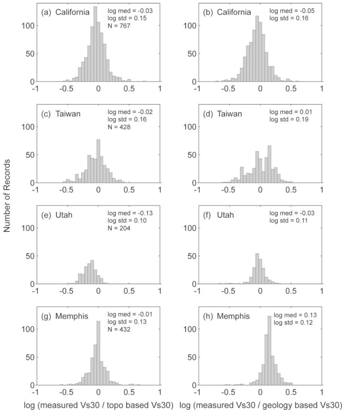
Figure 3. Histograms indicating logarithmic differences of measured V_{s30} values compared with values derived from topographic slope correlations (a, c, e, and g) or based on existing V_{s30} site-condition maps (b, d, f, and h). N is the number of V_{s30} measurements.
